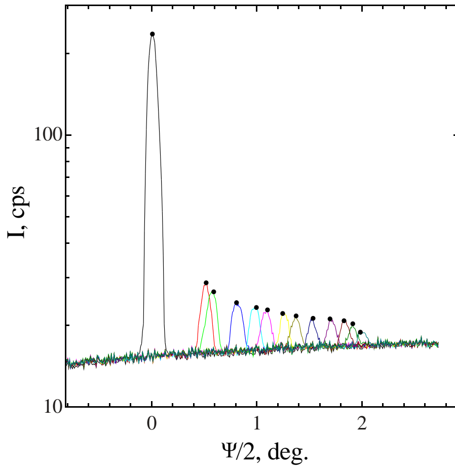
Fig. 5. Integral count-rate accounting a noise of the detector along Oy -axis as a function of the scattering angle \psi / 2 , (highest black curve) for the direct beam; (various color shapes) for the multiple successive reflections from the concave silica sol surface.
